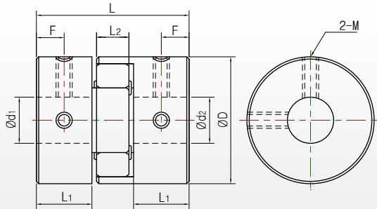
Out Diameter size \varnothing 14 \sim \varnothing 30
