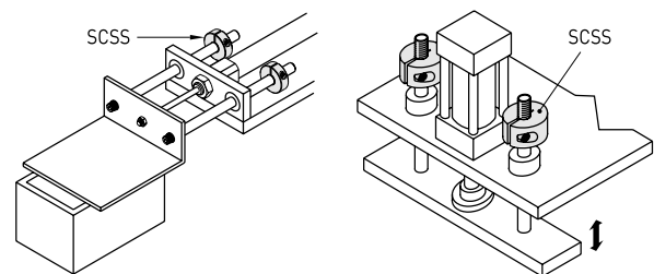
Example (Set Collars - Slit Type)
