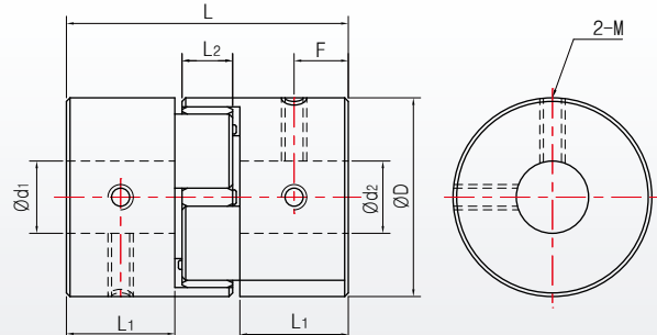
Out Diameter size \varnothing 40
